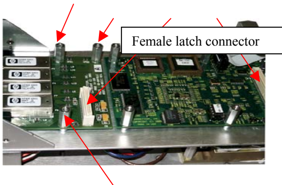
Fig 3.6.2c Granddaughter Board placed in slot & secured with three 5/16 standoff's
